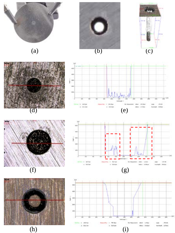
Fig. 5: through hole and the figures with relevant profiles under different parameters. (a) workpiece with through hole; (b) through hole; (c) 3D model; (d&e) small end of the hole and the profile generated; (f&g) big end of the hole and the profile generated; (h&i) big end of the hole and the profile generated with smartflash open.
