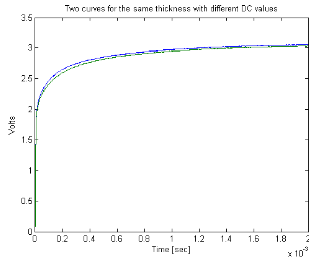
Figure 3. Example of two transitory waveforms for the same thicknesses of the Inox 304 material.
