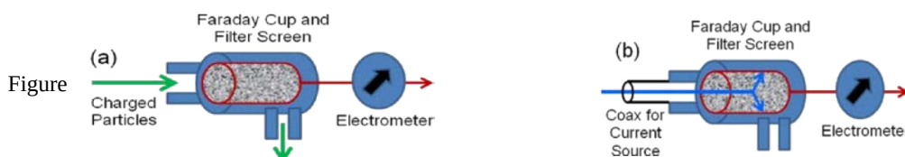
1. Charged particles (a) or known currents (b) are sourced to the Faraday cup of the aerosol electrometer.
