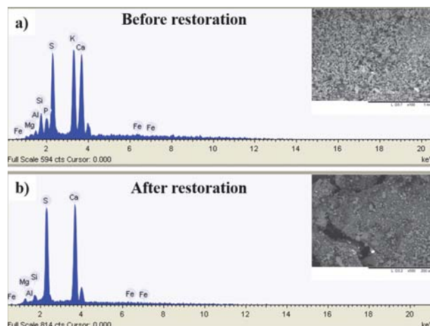
Fig. 4. Representative SEM-EDS analysis performed on sample; a) P3 (before restoration); b) P3a (after restoration)
