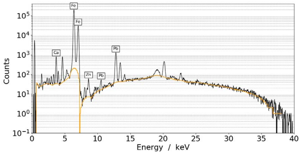
Fig. 2. XRF spectrum acquired on one of the pincers; the computed spectrum background is plotted in yellow. The identified material is an iron alloy.
