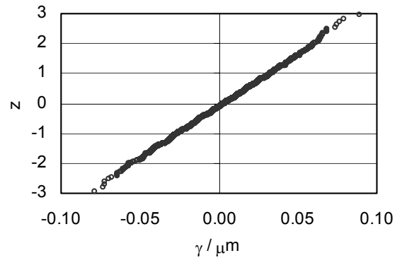
Figure 4: Normal probability plot of the empirical distribution of \hat{\gamma}_n^{ML} based on 1000 sample. The data for the Monte Carlo study have been generated as reported for figure 3.
