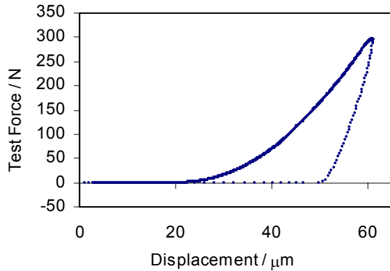
Figure 1: Force/Displacement characteristic curve obtained during an Instrumented Indentation Test (HM 300/54/550 = 6800 N/mm 2 ).
