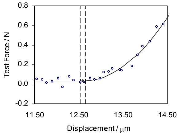
Figure 5: Experimental data (o) fitted by segmented regression curve (-). The maximum likelihood estimate of the abscissa of the zero-point is 12.60 \mu\text{m} and its 95% confidence interval is (12.54; 12.66) \mu\text{m} (-.-).
