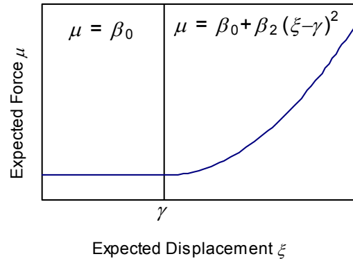
Figure 2: Force/Displacement Curve: segmented polynomial model used to fit the measured data in the neighbourhood of the zero-point ( \gamma is its abscissa).
