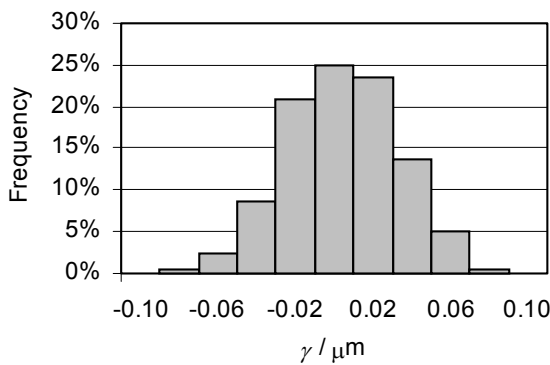
Figure 3: Histogram of the empirical distribution of \hat{\gamma}_n^{ML} based on 1000 sample. The data for the Monte Carlo study have been generated using the model (5) with \boldsymbol{\theta} = (0,0,0.1837)^T . Measurement errors have been considered independent and normally distributed with a standard uncertainty on the depth equal to 0.015 \mu\text{m} and a standard uncertainty on the force equal to 0.03 \text{ N} .
