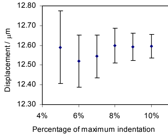
Figure 6: 95% confidence intervals of the abscissa of the zero-point calculated involving different percentages of maximum indentation depth. The uncertainty decreases with the increase of indentation depth used for the fitting.
