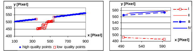
Fig. 8. Left: Measured contour points with probing direction from bright to dark, Right: fitted lines for all four calculations listed in Table 3
