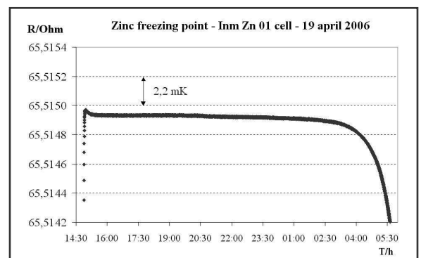
Fig. 4. Zinc freezing curve of the Inm Zn 01 cell
