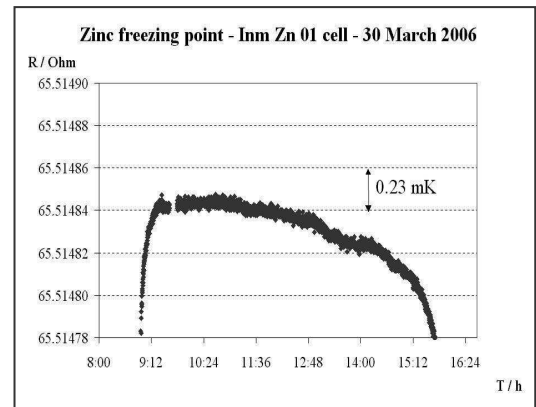
Fig. 5. Zinc freezing point curve of the Inm Zn 01 cell
