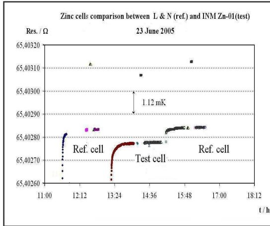
Fig. 7. Zinc freezing point curve of the Inm Zn 01 cell
