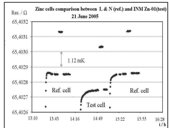
Fig. 6. Zinc freezing point curve of the Inm Zn 01 cell
